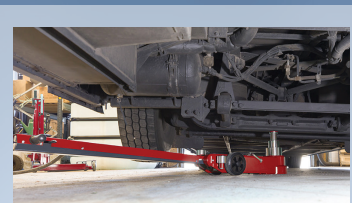
SKFW1 Floor-Jack V-Shaped Adapter Designed for lifting under various types of axles. 22,000 lbs. capacity
