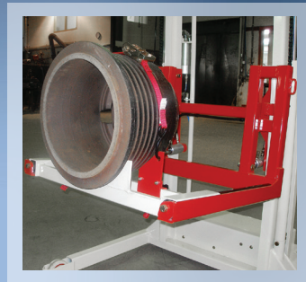
SKWD 500 shown with optional G-BDA brake drum adapter
